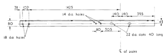
DETAIL 'A'—80 x 80 x 10 Angles.
