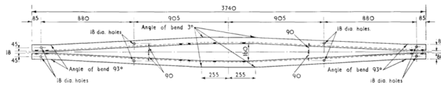
DETAIL 'D'-80 x 80 x 10 Angles.
