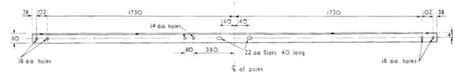
DETAIL 'C'-80 x 80 x 10 Angles
