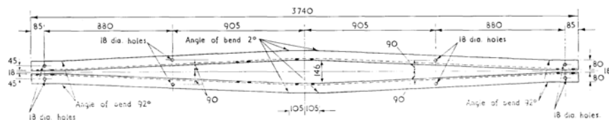
DETAIL 'A'—80 x 80 x 10 Angles.
