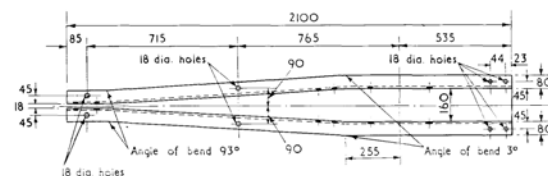
DETAIL B'-80 x 80 x 10 Angles.
