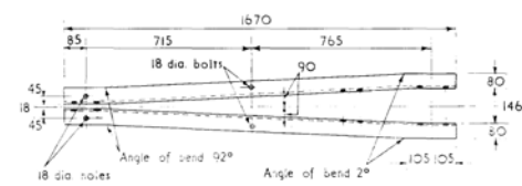
DETAIL 'C'-80 x 80 x 10 Angles
