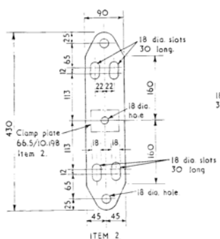
For use at earthwire section positions. Material :- 90 x 15 Flat Bar.
