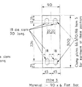
Material :- 90 x 6 Flat Bar.
